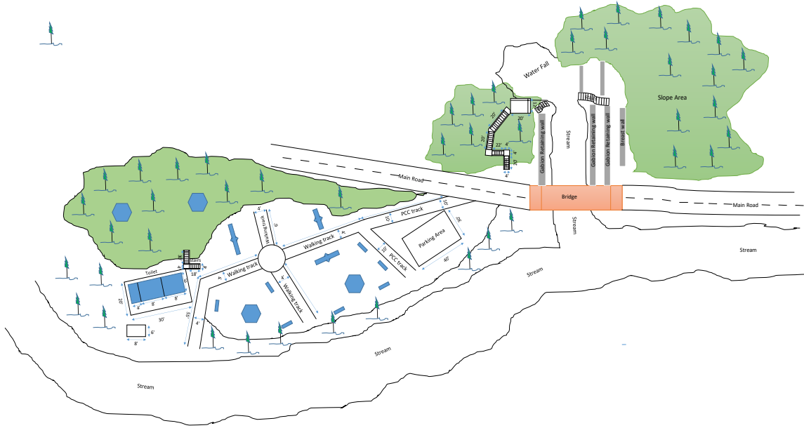
Hillan (Rage) Water Fall Plan
