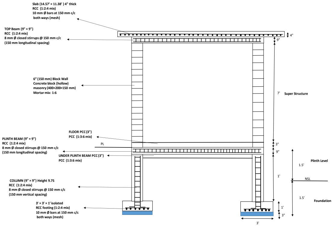
X-Section
