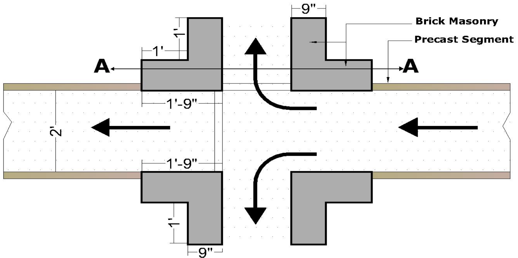
PLAN FOR THREE-WAY WATER TRANSPORT STRUCTURE (NAKKA)
