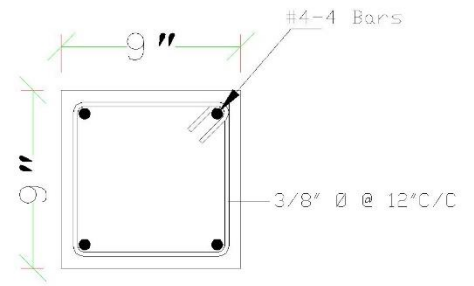
BEAM DETAIL
