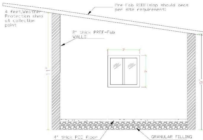
SECTION VIEW
