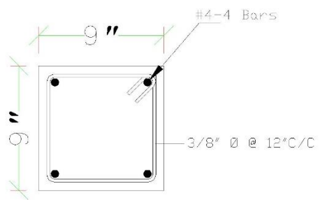
BEAM DETAIL
