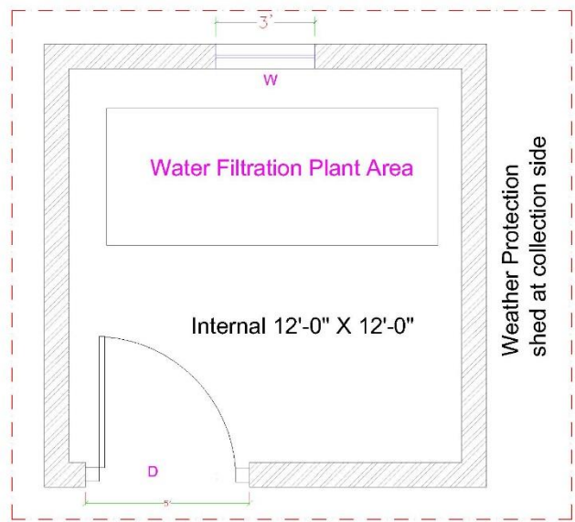
PLAN VIEW
