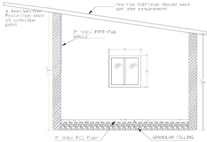
SECTION VIEW
